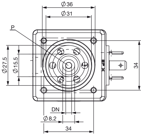
Subbase version
