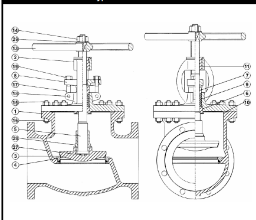
Typical Construction
