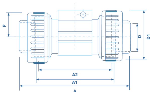
INLINE Sensor Fitting Dimensions
