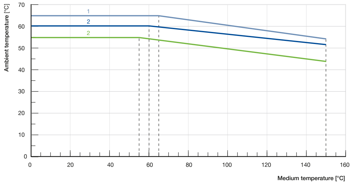
Temperature diagram AG2
